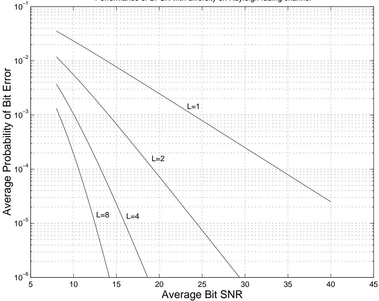
Performance of BPSK with diversity on Rayleigh fading channel
